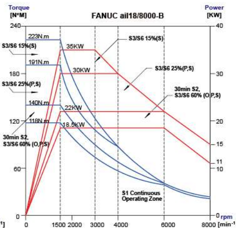
BT50 Belt type 8000rpm
