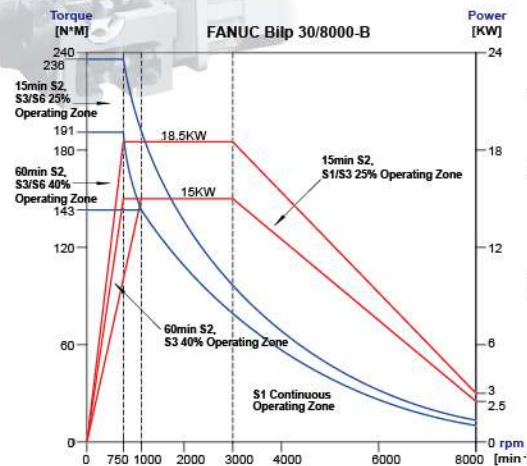
BT50 Belt type 8000rpm
