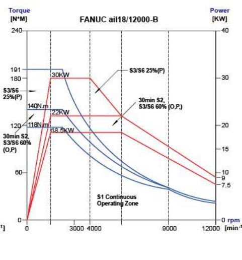
BT50 Direct type 10000rpm
